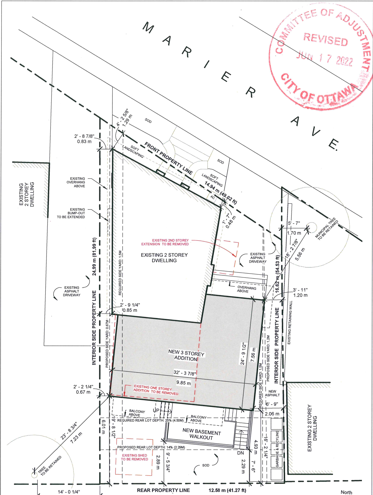
1 SITE PLAN 1/8" = 1'-0"
