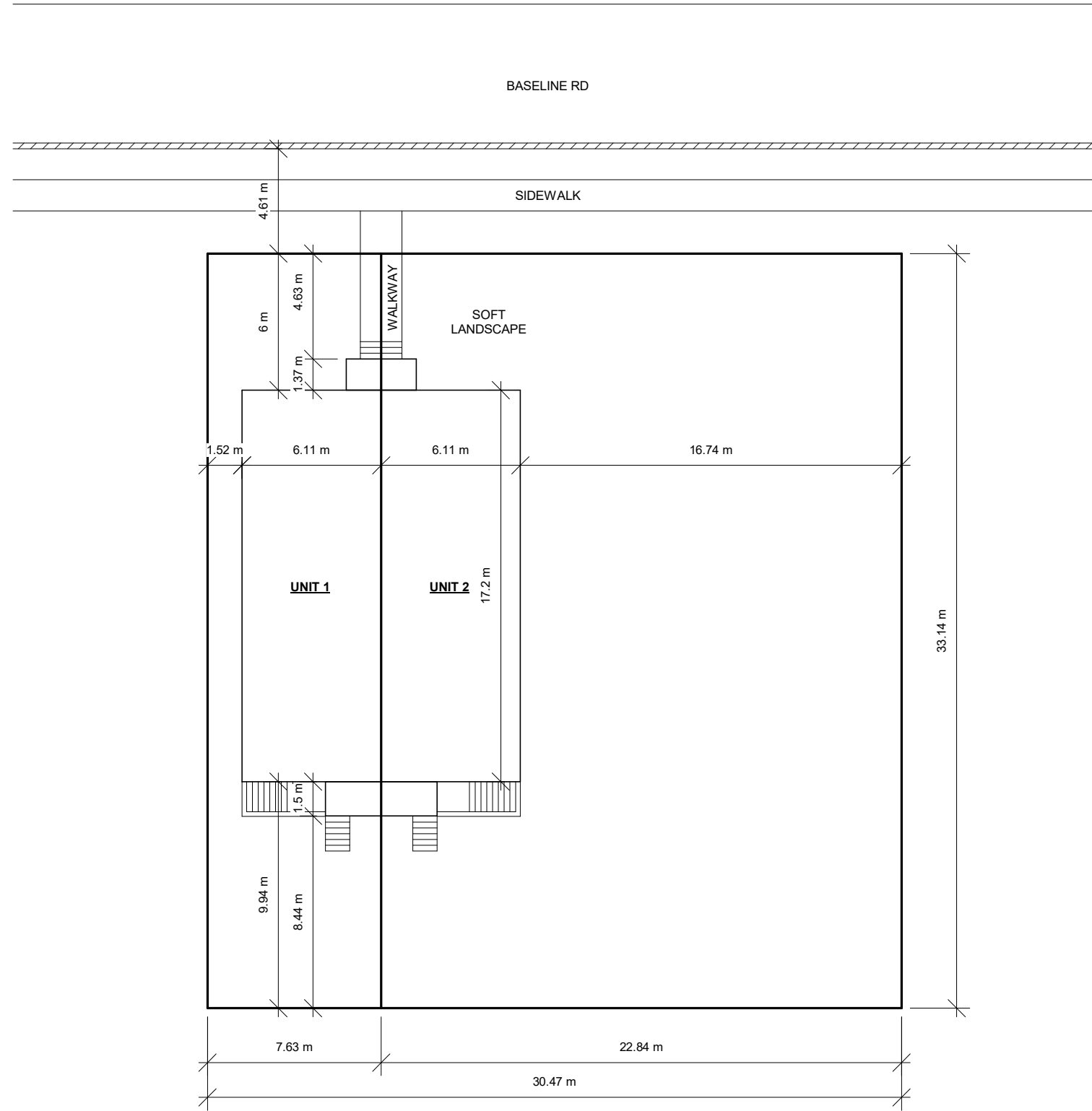
1 Site Plan 1" = 20'-0"
