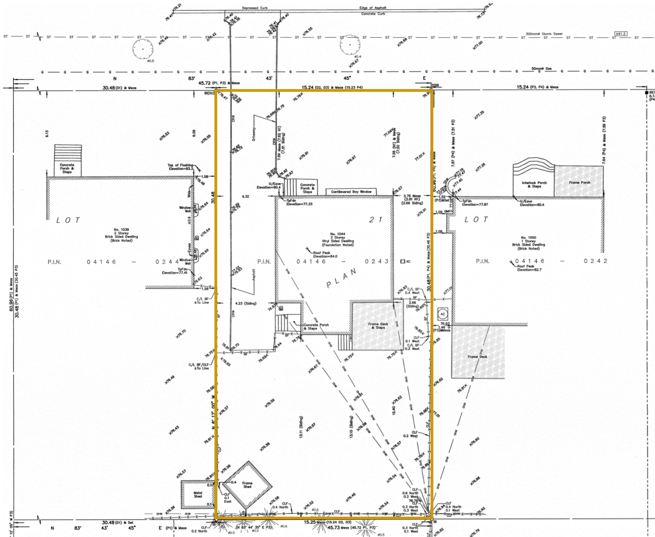
Figure 3. Extract of topographic survey prepared by Farley, Smith & Denis Surveying Ltd.
