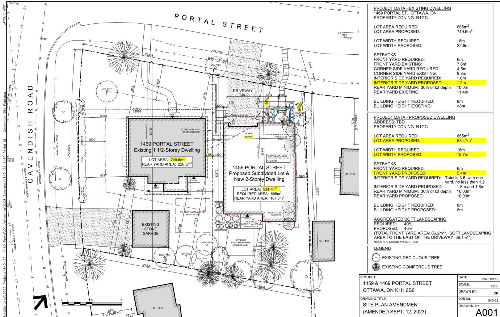
Figure 2-1: Site Plan (Excerpt), prepared by Simmonds Architecture (dated September 12, 2023)
