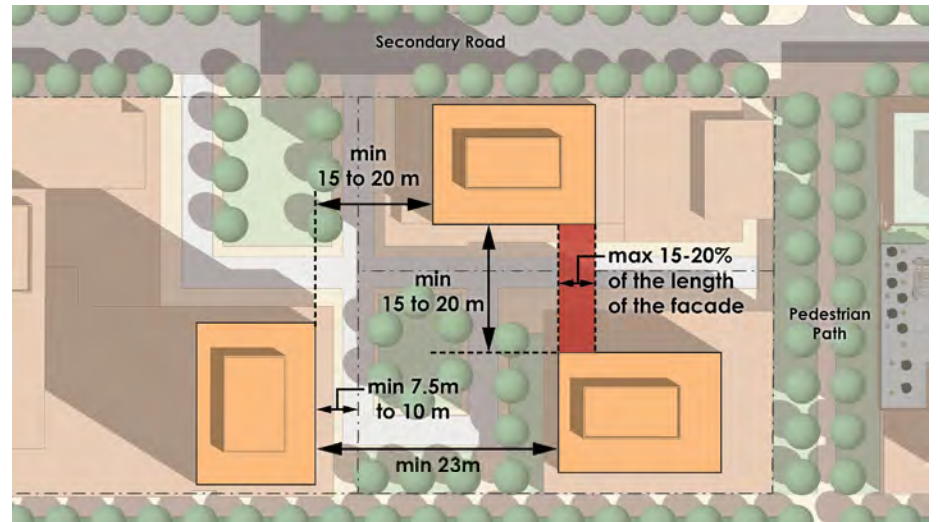
(Figure 3.6) A conceptual illustration showing the proper tower spacing distances.
