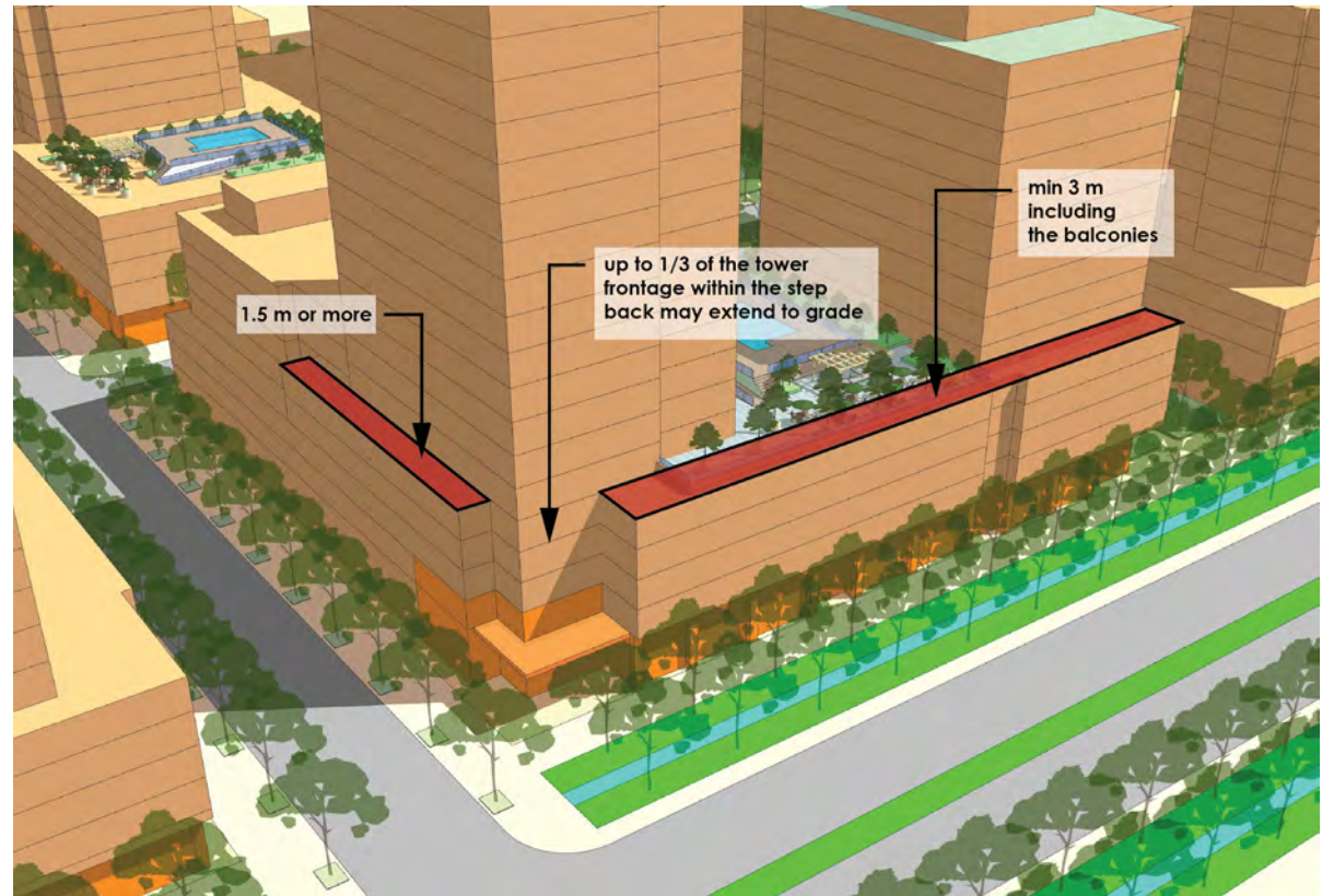
(Figure 3.7) A conceptual illustration of the required building step backs.
