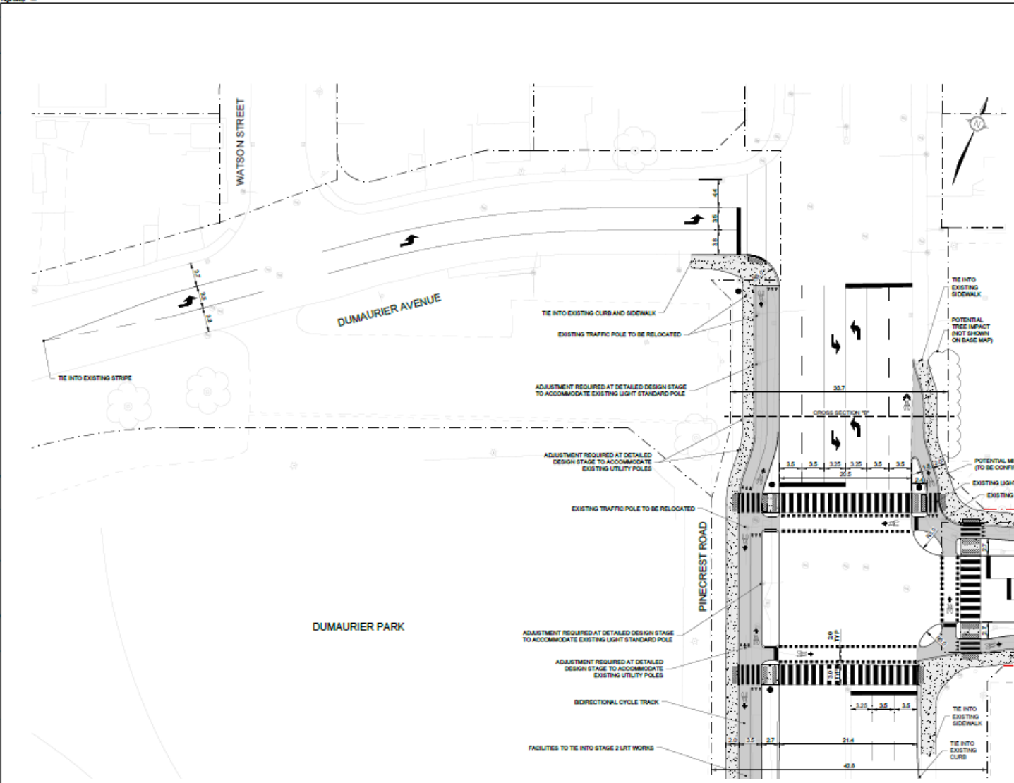
PLAN 1 - PINECREST ROAD AT DUMAURIER AVENUE/QUEENSVIEW DRIVE 1:250
