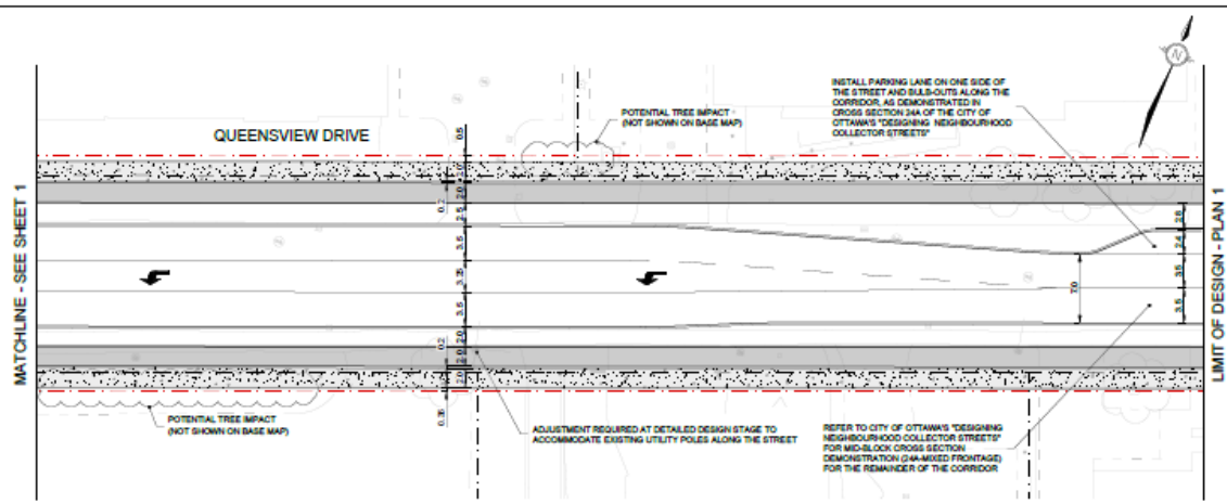
PLAN 1 - QUEENSVIEW DRIVE (CONTINUATION) 1:250
