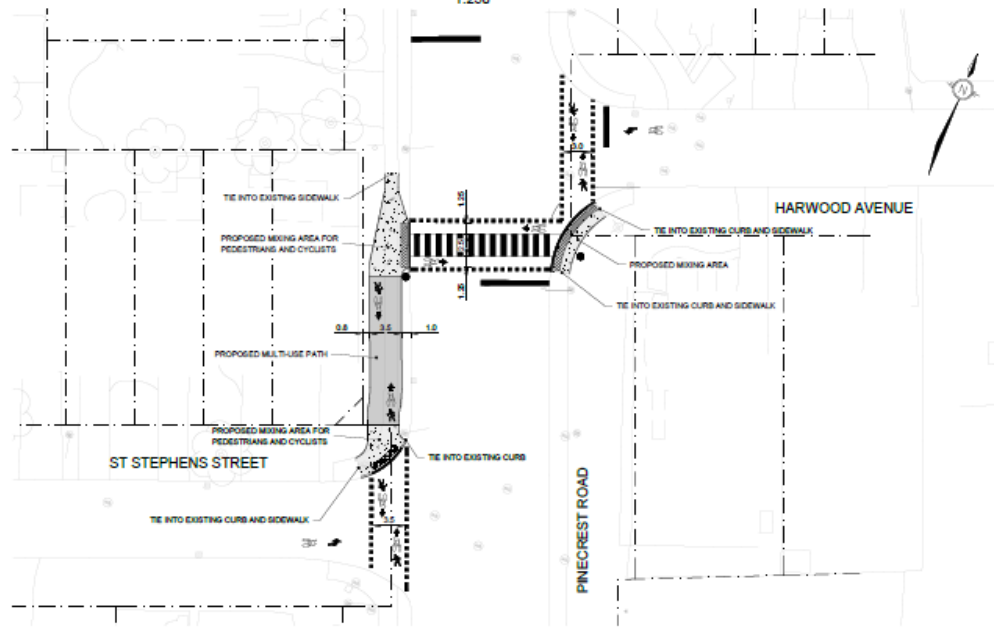
PLAN 2 - PINECREST ROAD CROSSING AT HARWOOD AVENUE 1:250
