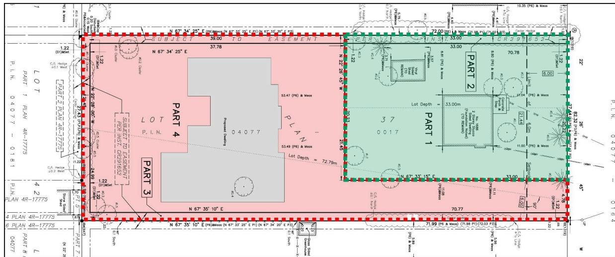
Fig.7.Draft 4R plan showing the severed and retained lands by Farley, Smith & Denis Surveying LTD, 2025
