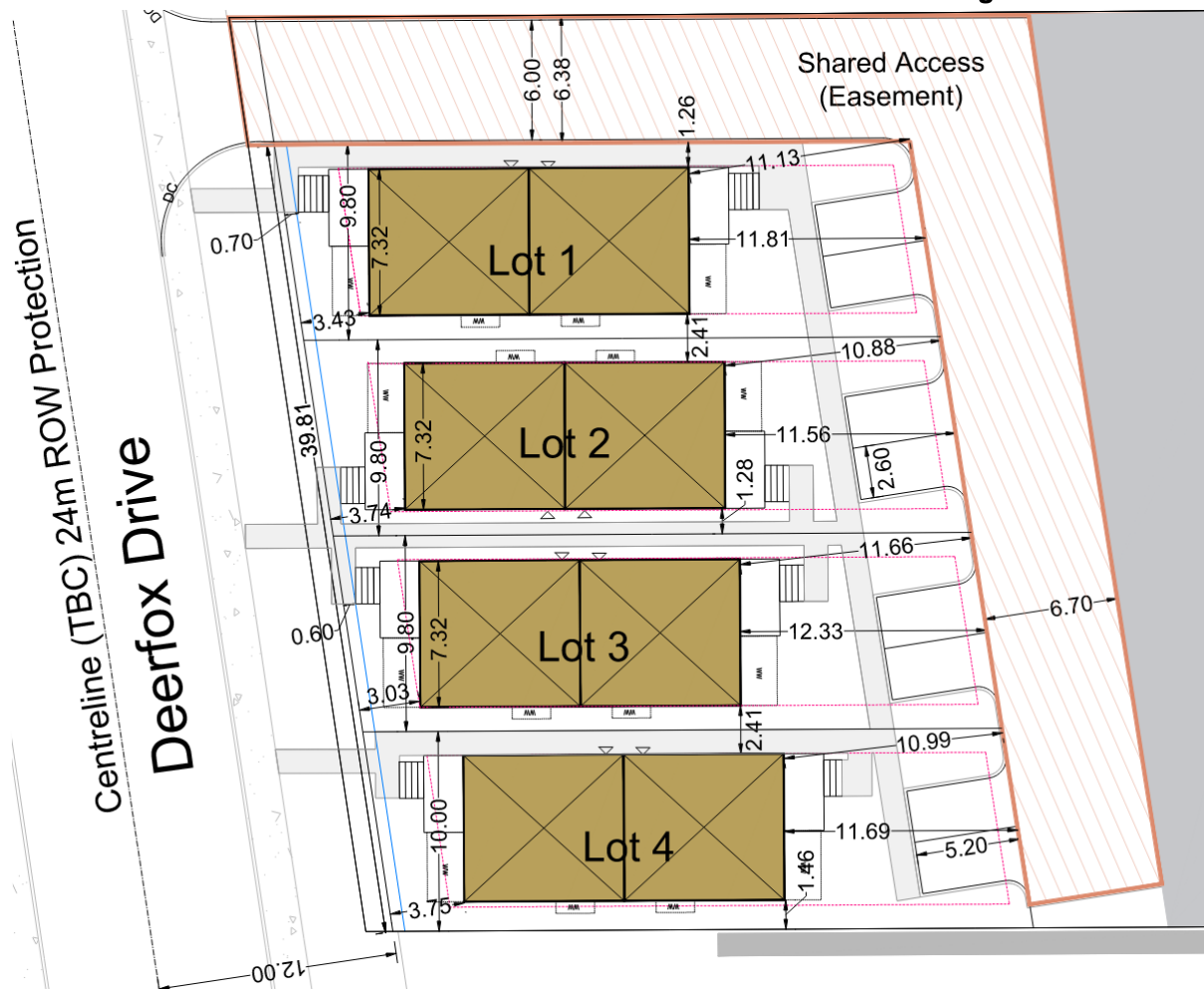
Figure 2. Site Plan
