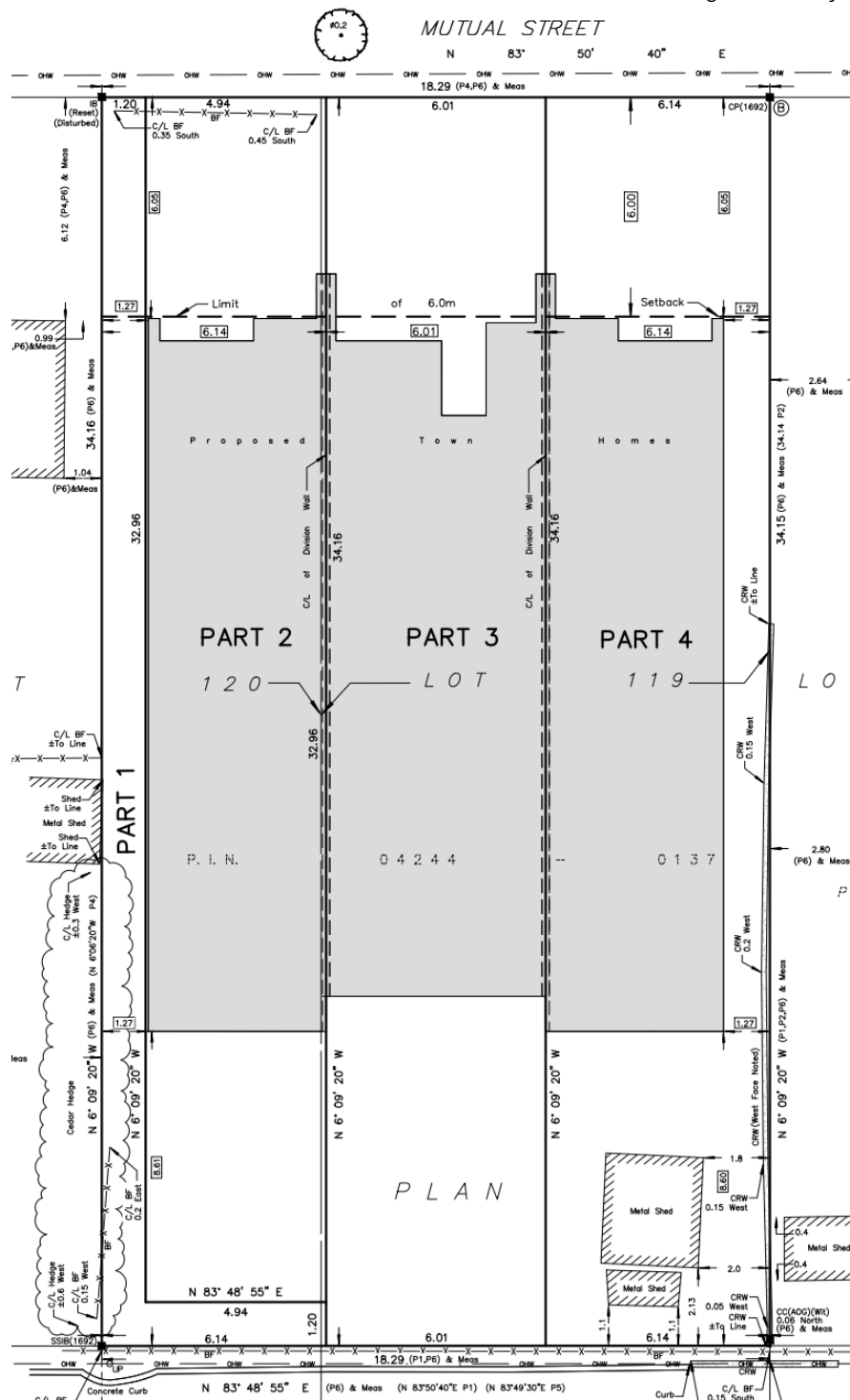
Figure 1: Draft Reference Plan Excerpt
