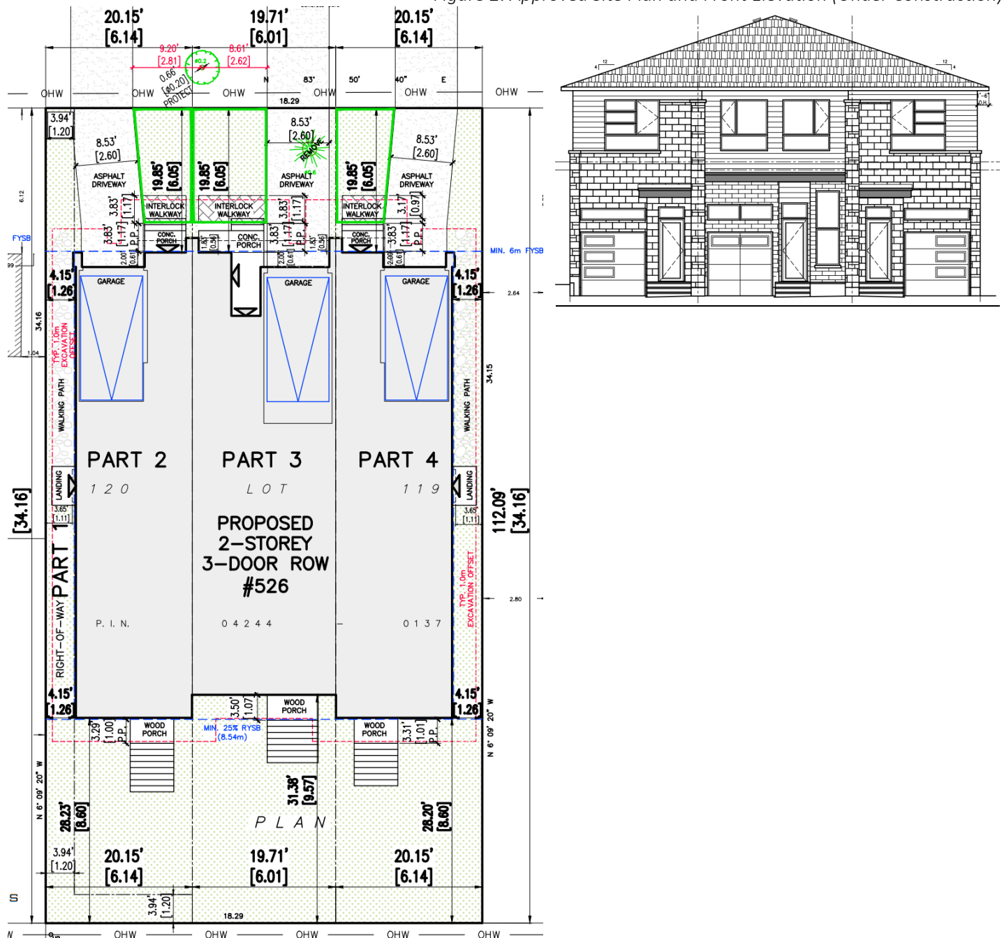
Figure 2: Approved Site Plan and Front Elevation (Under Construction)
