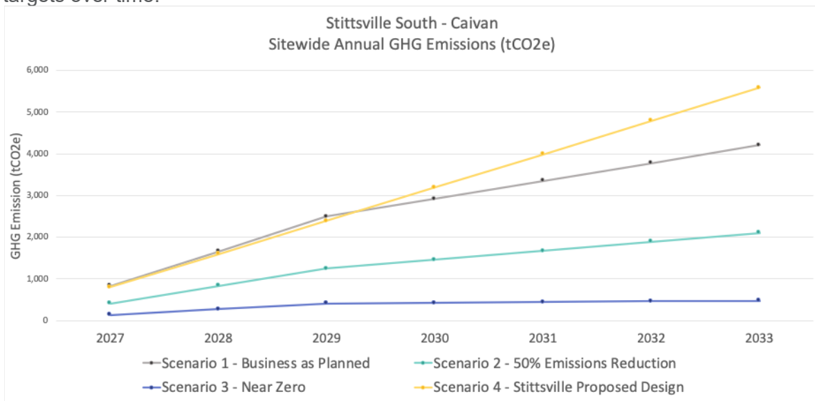
Figure 5: Stittsville South Sitewide GHGI for Scenarios 1-4 (KgCO 2 e/m 2 )
