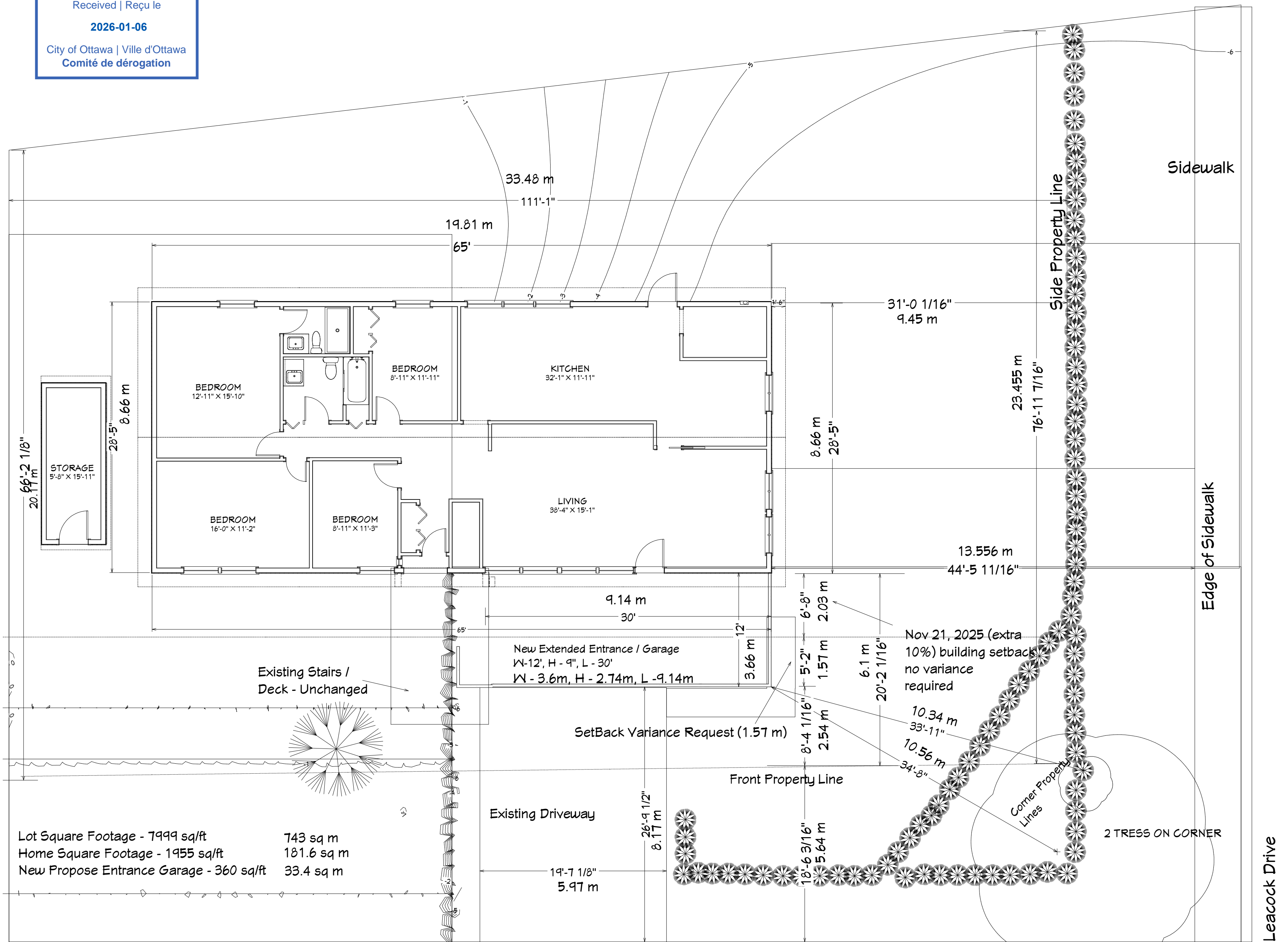
43 Pentland Cres - Site Plan
