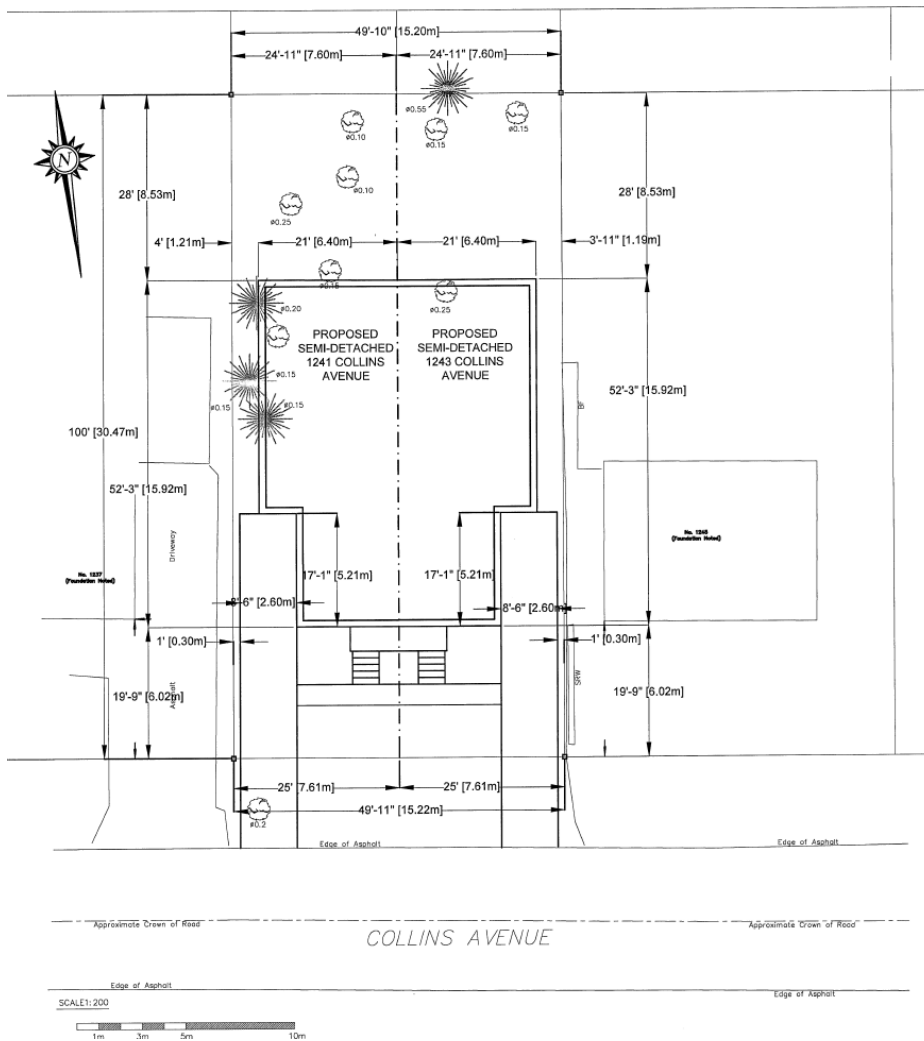
Figure 1- Site Plan
