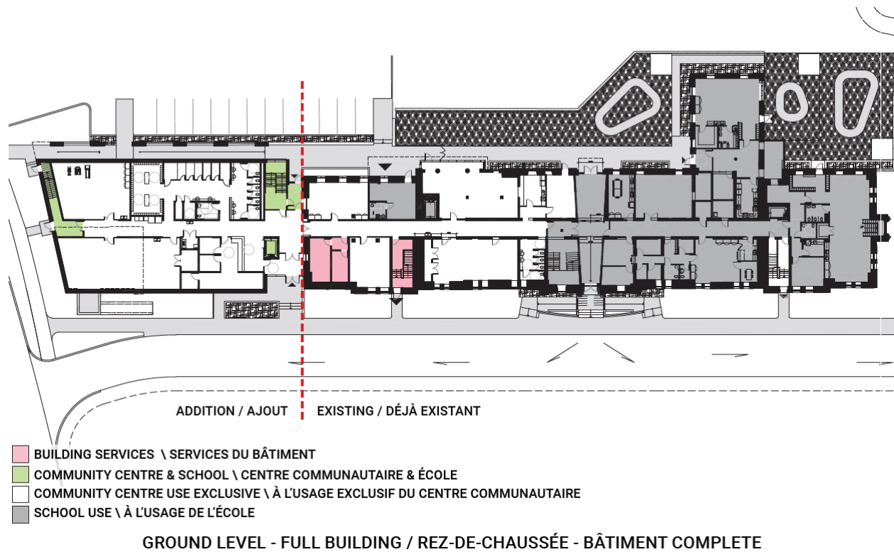
Figure 3 - Outline Drawings
