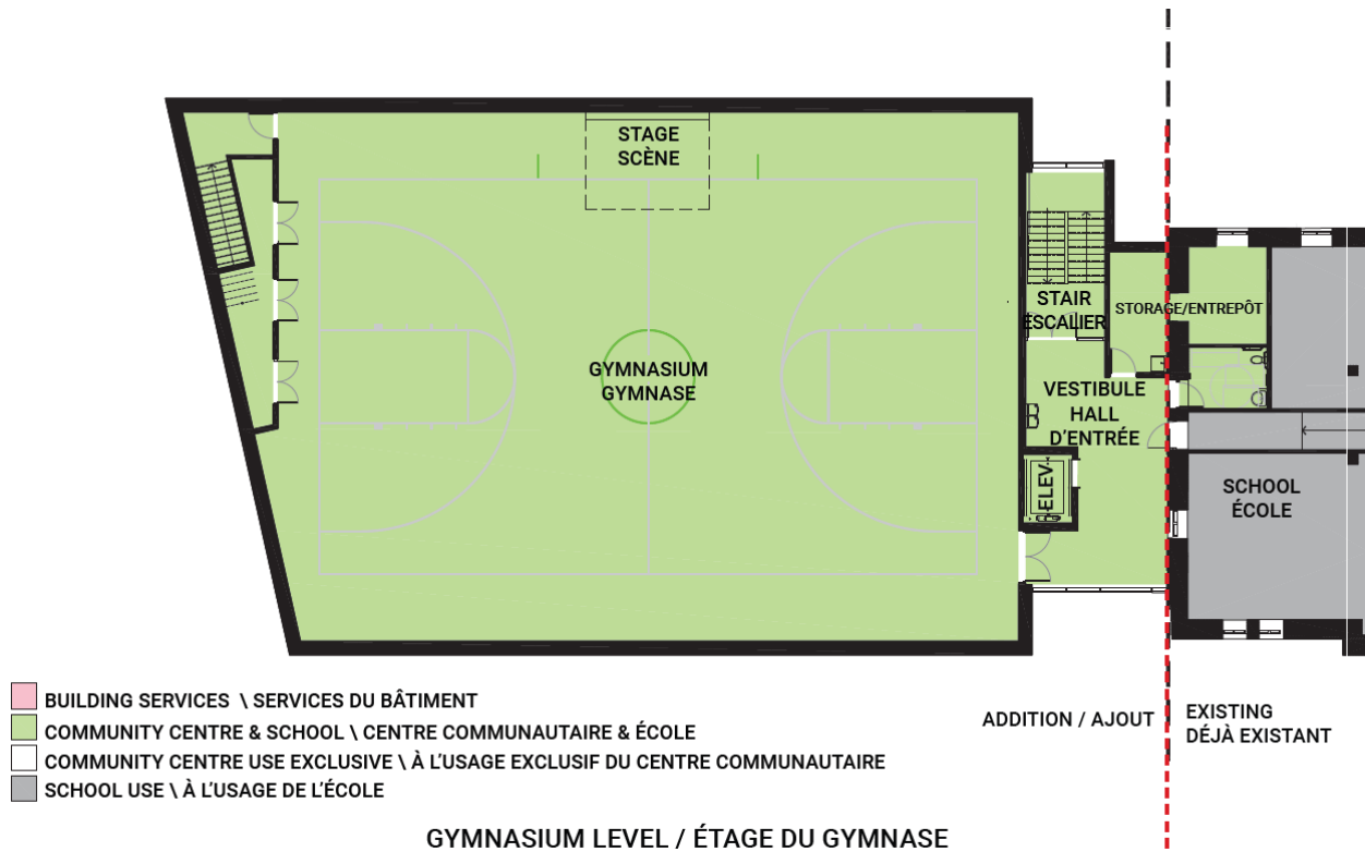
Figure 7 - Outline Drawings
