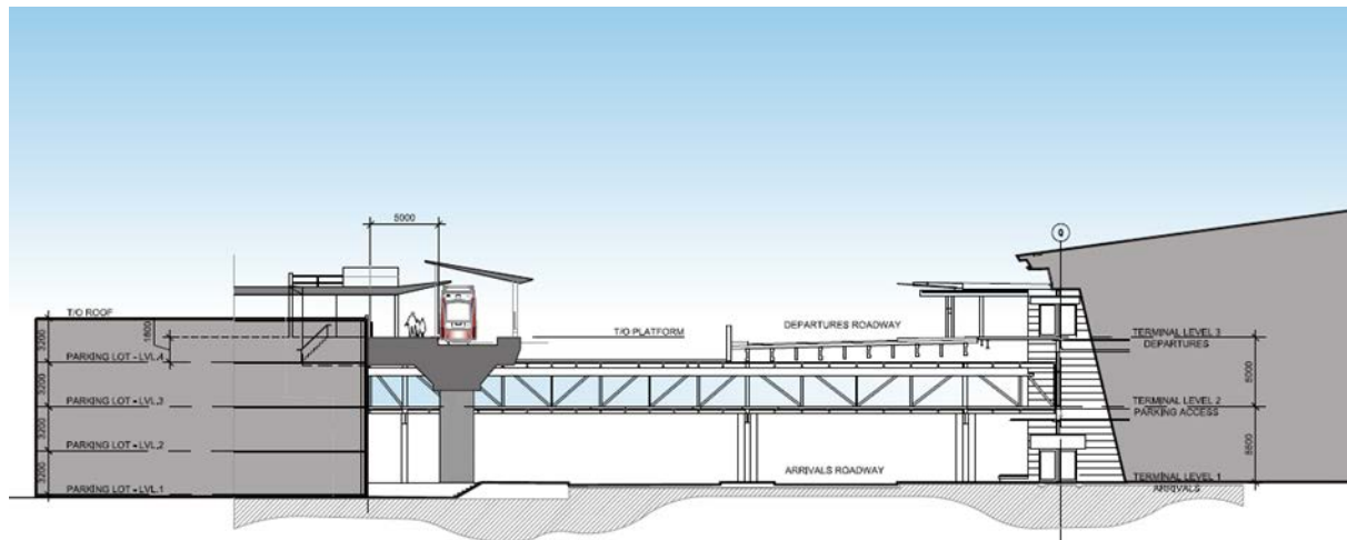
Figure 23: Terminal Station
