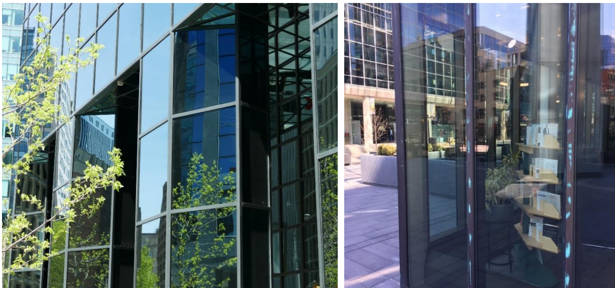
Figure 8: Potential design traps (mirror maze and black hole effect on left, corner glass on right).
